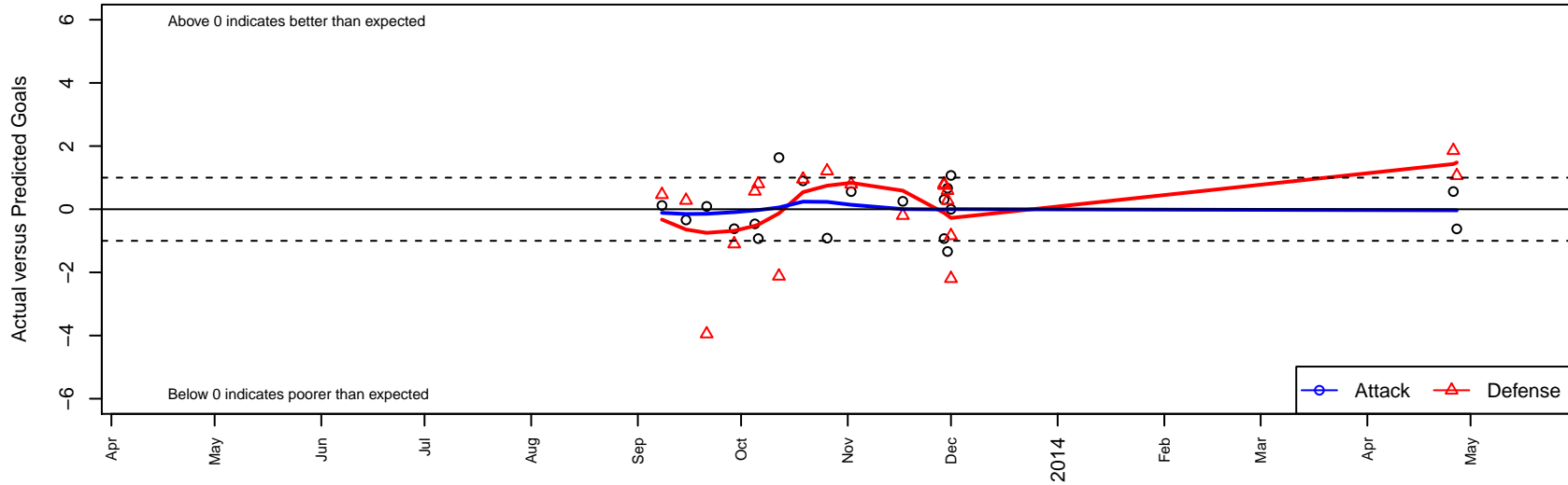
FC Manchester United Red B99 Dots are actual minus expected GF (blue circles) and GA (red triangles). Blue line is smoothed change in attack strength. Red is smoothed change in defense strength.
